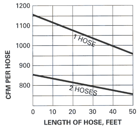
F33 WITH SOURCE CAPTURE PLENUM AND 8" HOSE
